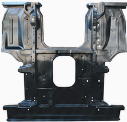
VETK 279 Flooring (Assy.)
